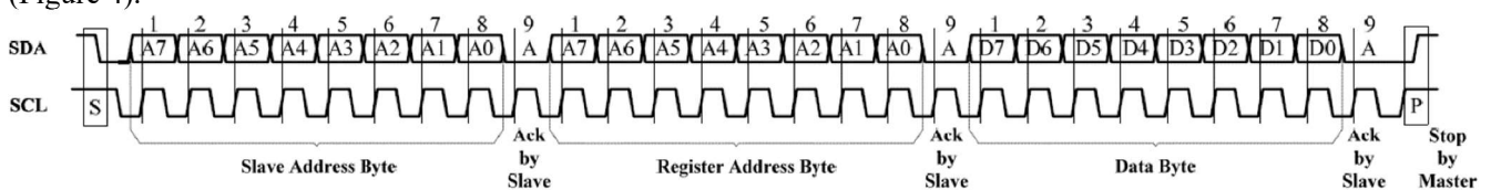
Figure 3 Typical I 2 C Writing
