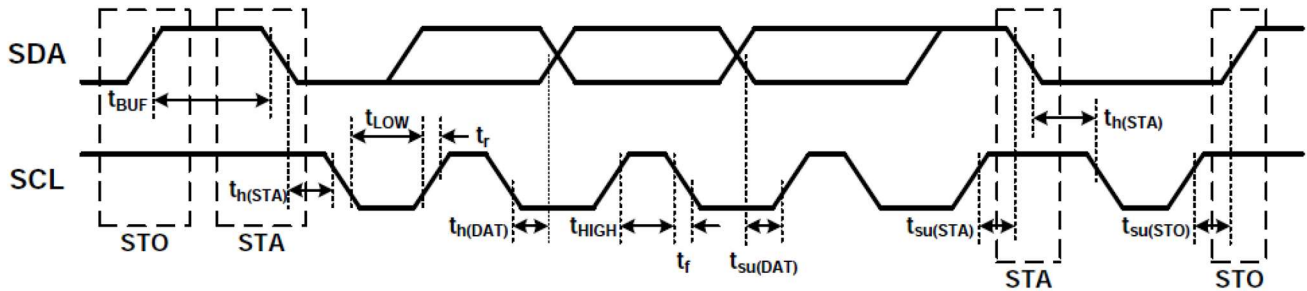
Figure 1 I 2 C Interface Timing
